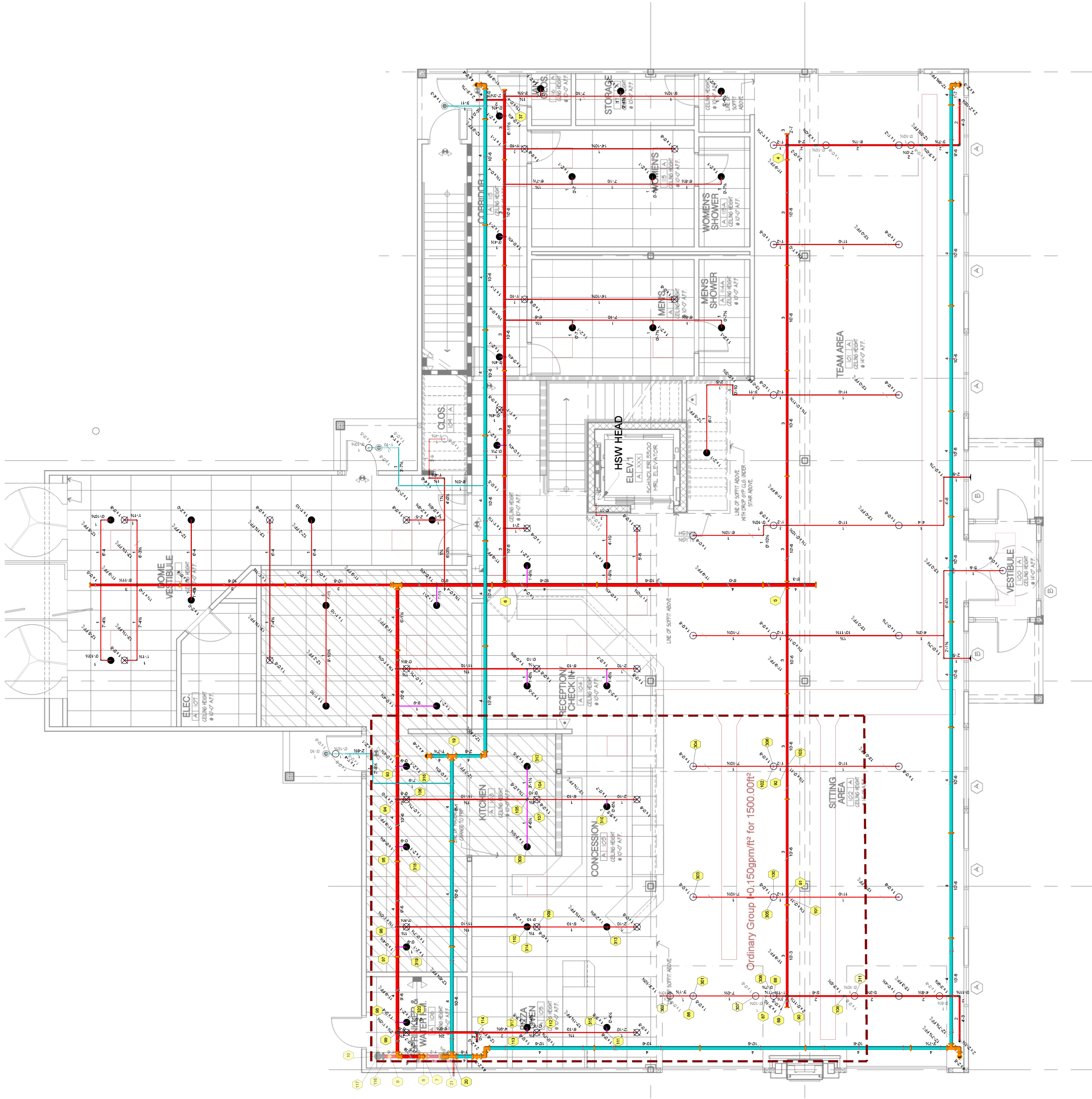
1st FLOOR FIRE SPRINKLER PLAN SCALE: 3/16" = 1'-0"
